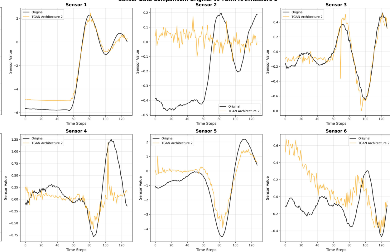
Sensor Data Comparison: Original vs TGAN Architecture 2
