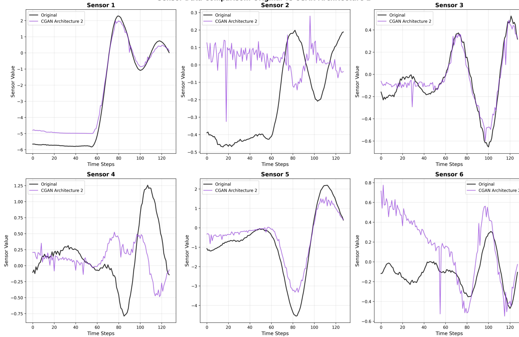
Sensor Data Comparison: Original vs CGAN Architecture 2
